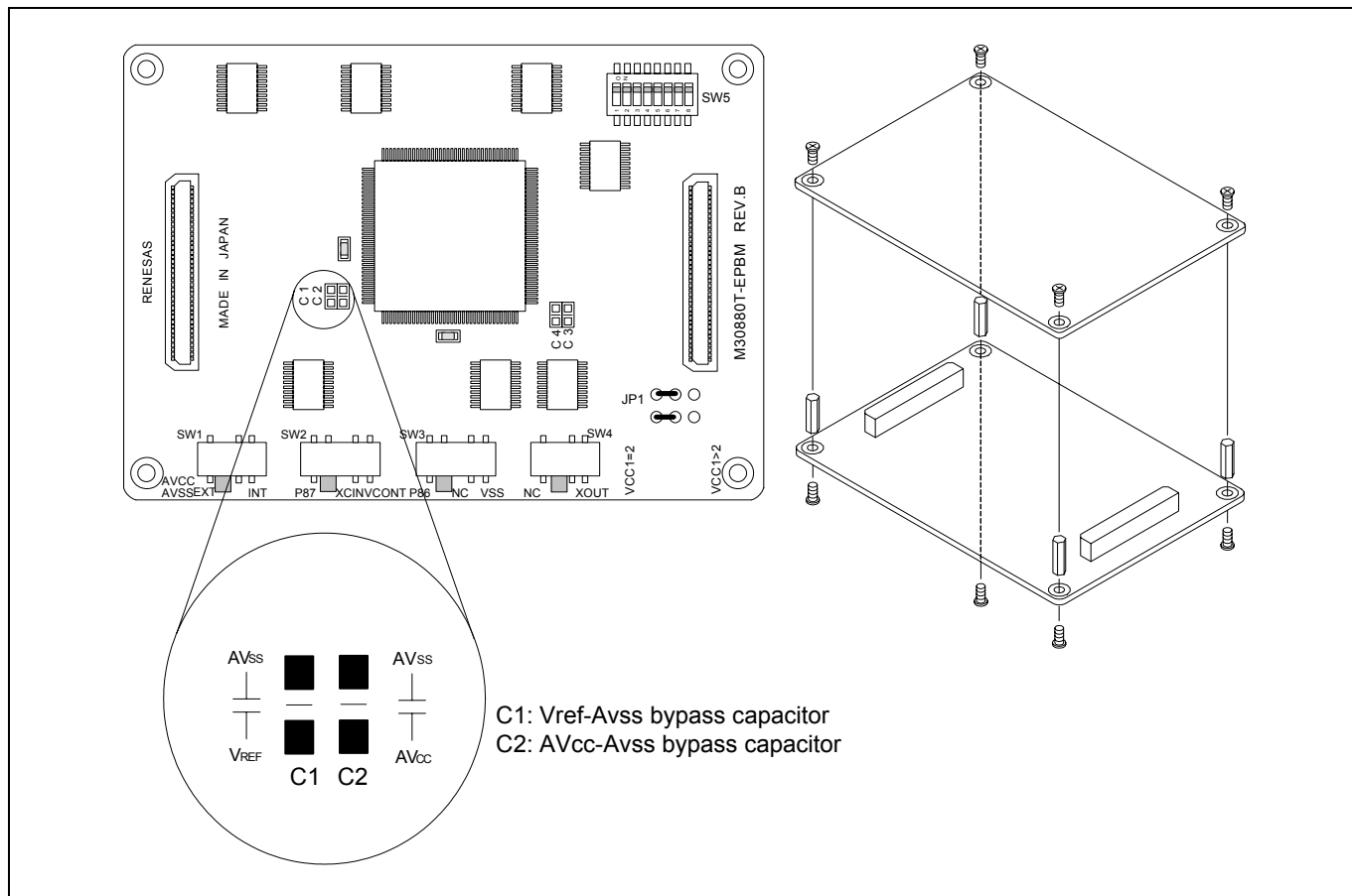
Figure 2.23 Foot pattern for the A/D conversion bypass capacitor
